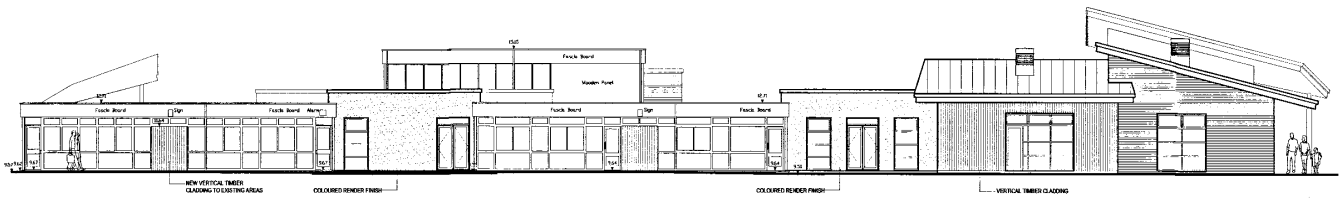
PROPOSED SOUTH ELEVATION - facing "Tree Belt"
