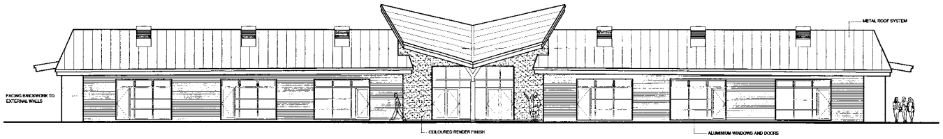
PROPOSED EAST ELEVATION - showing New Extension
