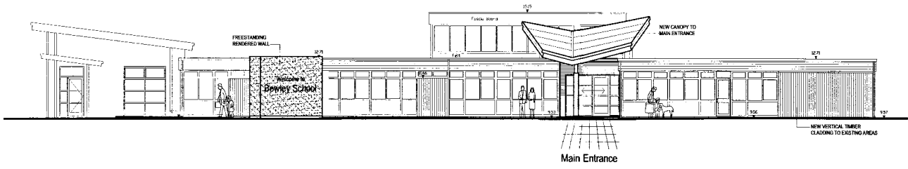
PROPOSED WEST ELEVATION (to Main Entrance) - facing Low Grange Avenue
